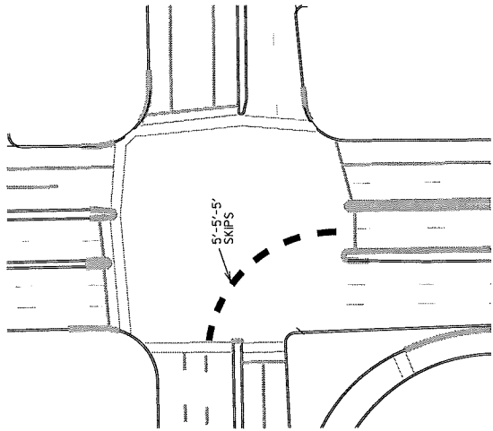
TURN RADIUS LINE DETAILS
